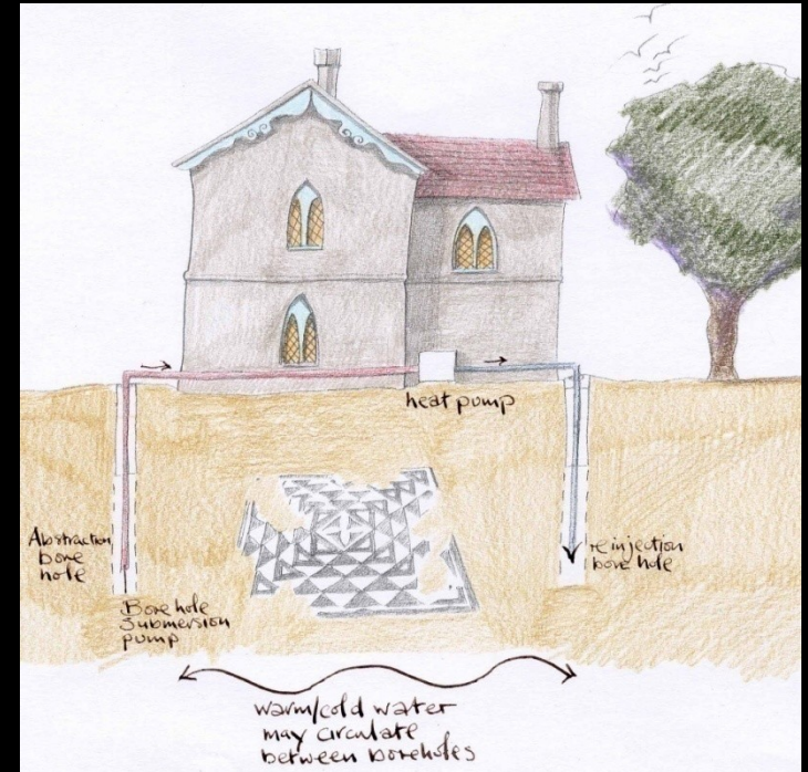
Open Loop System
